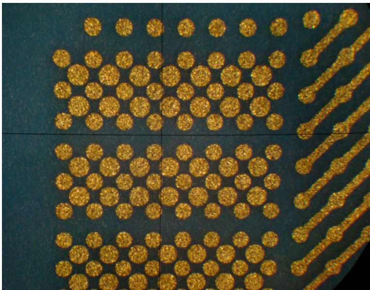
100 μm and 120 μm pads with 20 μm spaces
